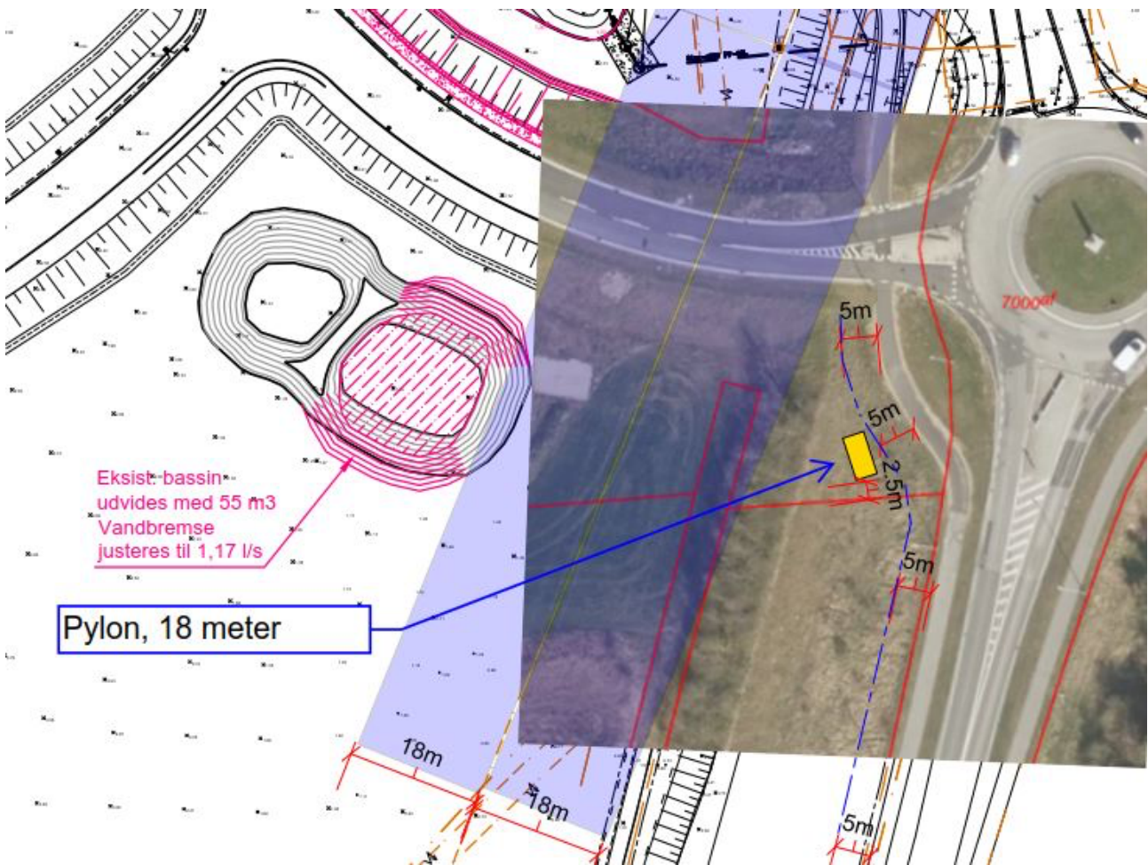
Figur 1: Situationsplan - Pylonplacering McDonald's Korsør
