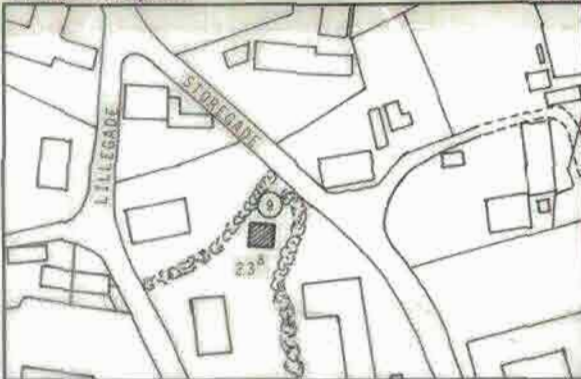
Situationsplan 1:2000
