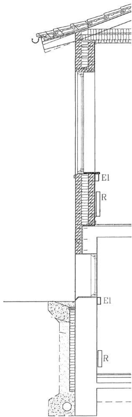
DETAIL-SNIT L1
